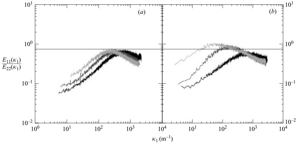
FIGURE 23. Energy spectra ratio, downstream evolution. (a) 2.54 cm passive grid, short precontraction (1PS), R_{\lambda_a} = 40 , \bar{S} = 12 ; (b) active grid, random mode, short pre-contraction (RS), R_{\lambda_a} = 260 , \bar{S} = 24 . Black line, station b; dark grey line, intermediate station; light grey line, station e. The horizontal line is the ratio in the inertial subrange for isotropic turbulence.
