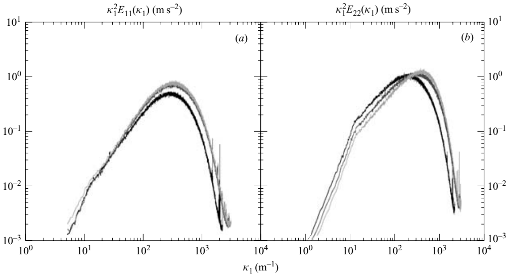
FIGURE 21. One-dimensional dissipation spectra, downstream evolution, 2.54 cm passive grid, short precontraction (1PS), R_{\lambda_1} = 40 , \bar{S}^* = 12 . (a) \kappa_1^2 E_{11}(\kappa_1) ; (b) \kappa_1^2 E_{22}(\kappa_1) ; black line, station a ; dark grey line, intermediate station; light grey line, station e .
