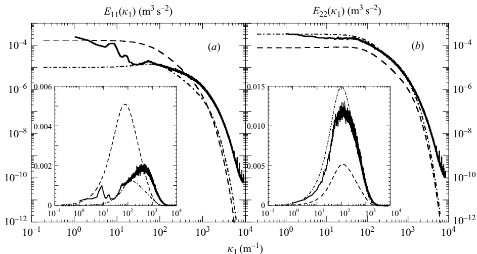
FIGURE 13. One-dimensional energy spectra, 2.54 cm passive grid, short precontraction (1PS), R_{\lambda_a} = 44 , \bar{S}^* = 12 . This is the same condition as shown in figure 10. Here the purpose is to compare with the RDT predictions made by extrapolating the data to the immediate precontraction region (see text). (a) E_{11}(\kappa_1) , inset \kappa_1 E_{11}(\kappa_1) ; (b) E_{22}(\kappa_1) , inset \kappa_1 E_{22}(\kappa_1) . Dashed line, station a extrapolated model spectrum; thick black line, station b experiment; dashed-dotted line, station b extrapolated model spectrum. The postcontraction wavenumbers have been multiplied by c and the amplitudes of the spectra by 1/c .
