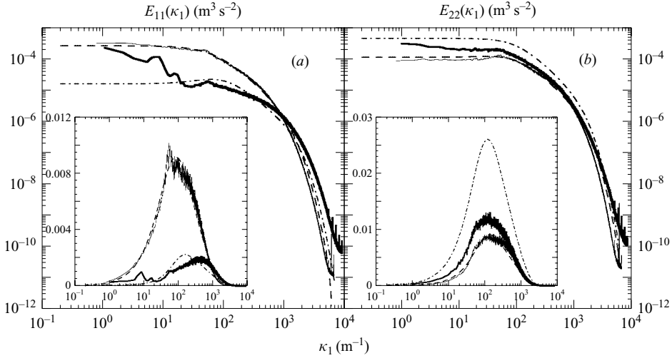
FIGURE 10. One-dimensional energy spectra, 2.54 cm passive grid, short precontraction (1PS), R_{\lambda_a} = 44 , \bar{S} = 12 . (a) E_{11}(\kappa_1) , inset \kappa_1 E_{11}(\kappa_1) ; (b) E_{22}(\kappa_1) , inset \kappa_1 E_{22}(\kappa_1) . Thin black line, station a experiment; dashed line, station a model spectrum. Thick black line, station b experiment; dashed-dotted line, station b model spectrum. The postcontraction wavenumbers have been multiplied by c and the amplitudes of the spectra by 1/c (see text immediately following (equation 2.27)).
