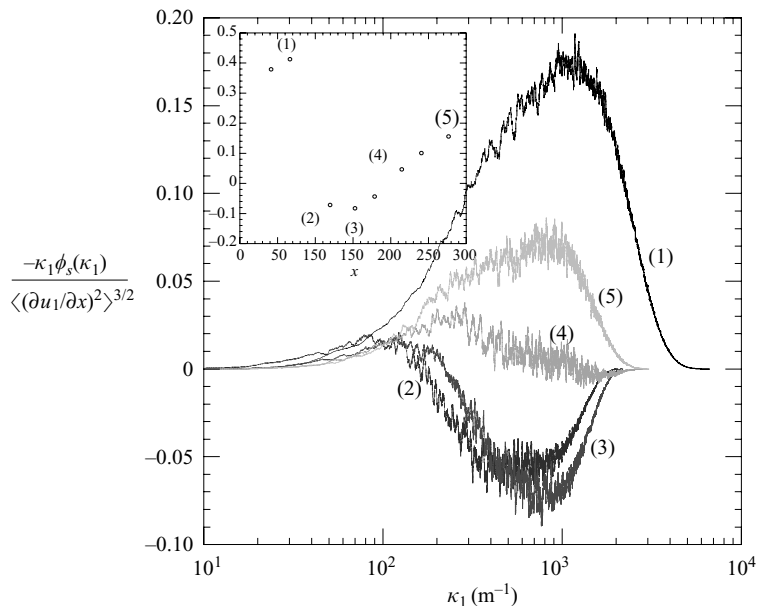
FIGURE 26. Skewness spectra -\kappa_1 \phi_s(\kappa_1) / \langle (\partial u_1 / \partial x)^2 \rangle^{3/2} , downstream evolution, 2.54 cm passive grid, short precontraction (1PS), R_{\lambda_1} = 44 , \overline{S}^* = 12 . (Inset shows the derivative skewness, -S_{\partial u_1 / \partial x} vs x .) (1) station a ; (2) station b ; (3) and (4) intermediate stations; (5) station e .
