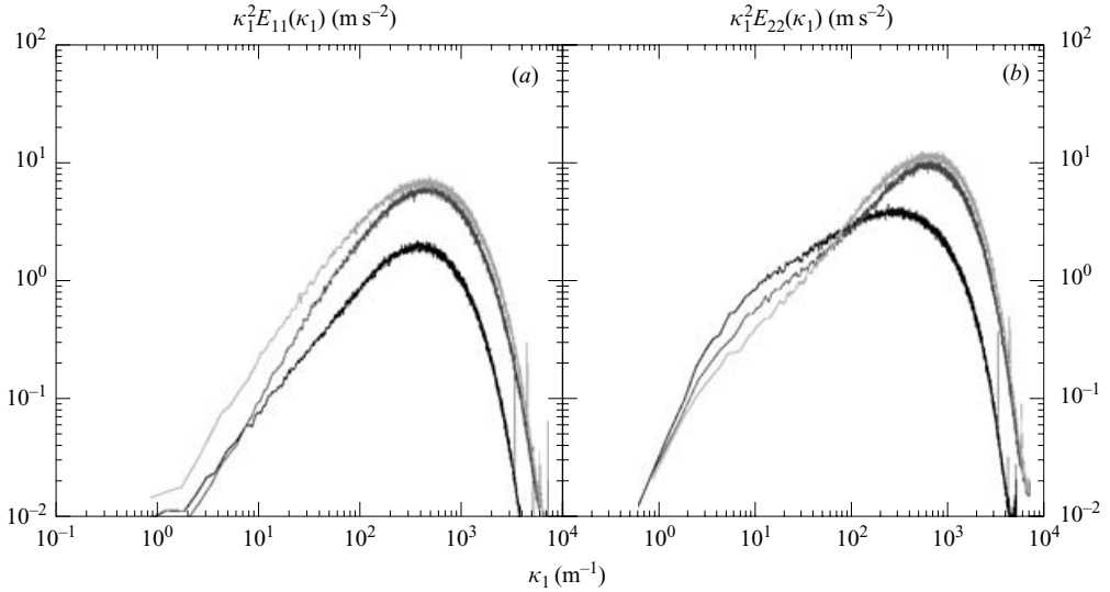
FIGURE 22. One-dimensional dissipation spectra, downstream evolution, active grid, long precontraction (RL), R_{\lambda_a} = 260 , \bar{S} = 24 : (a) \kappa_1^2 E_{11}(\kappa_1) ; (b) \kappa_1^2 E_{22}(\kappa_1) ; black line, station b; dark grey line, intermediate station; light grey line, station e.
