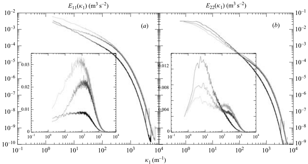
FIGURE 19. One-dimensional energy spectra, downstream evolution, active grid, long precontraction (RL), R_{\lambda_a} = 260 , \bar{S} = 24 . (a) E_{11}(\kappa_1) , inset \kappa_1 E_{11}(\kappa_1) ; (b) E_{22}(\kappa_1) , inset \kappa_1 E_{22}(\kappa_1) ; black line, station b ; dark grey line, intermediate station; light grey line, station e .
